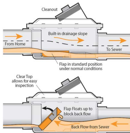
FIGURE 33. TYPICAL BACKFLOW PREVENTION VALVE DESIGNED TO PREVENT SEWAGE FROM BACKING FROM SEWAGE SYSTEM INTO PROPERTY. SOURCE: SQUARE ONE INSURANCE SERVICES, SQUAREONEINSURANCE.COM.
